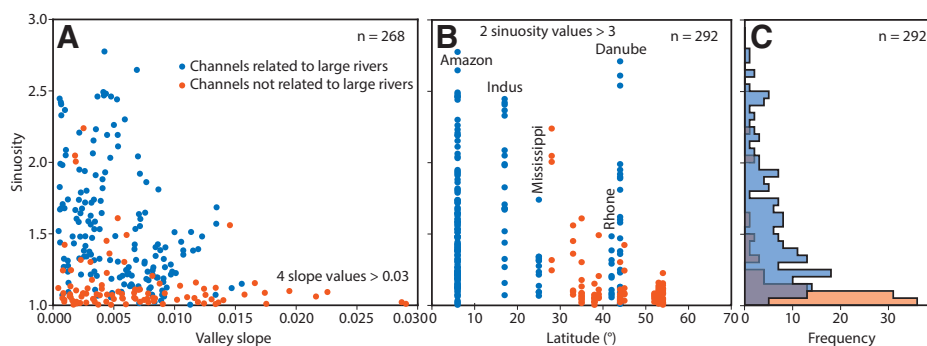
Figure 1. A: Scatterplot of sinuosity versus valley slope. B: Scatterplot of sinuosity versus latitude. C: Histogram of sinuosity values. Data sources same as in Table 1. Blue and orange colors show whether the channel is related to a large river (Indus, Mississippi, Rhone, Danube, and Amazon channels) or not (the rest of the data points).
